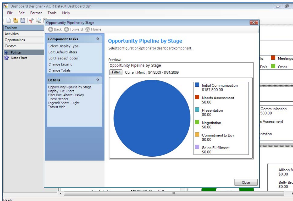
Figure 11: Dashboard Designer
