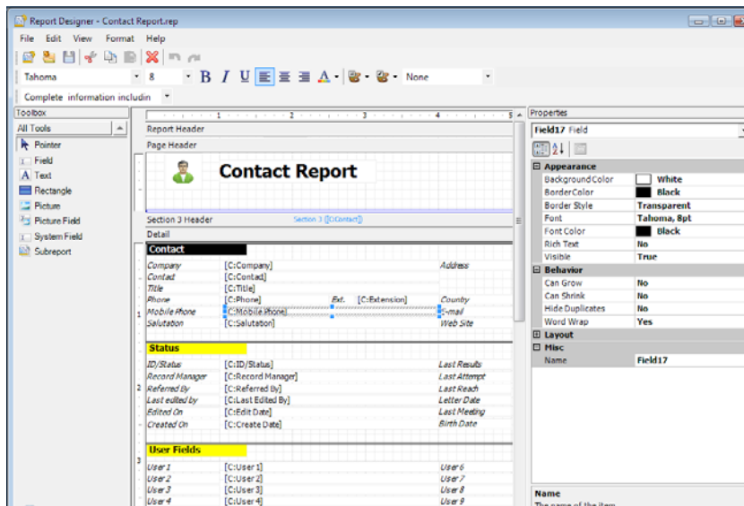
Figure 9: Report Design
