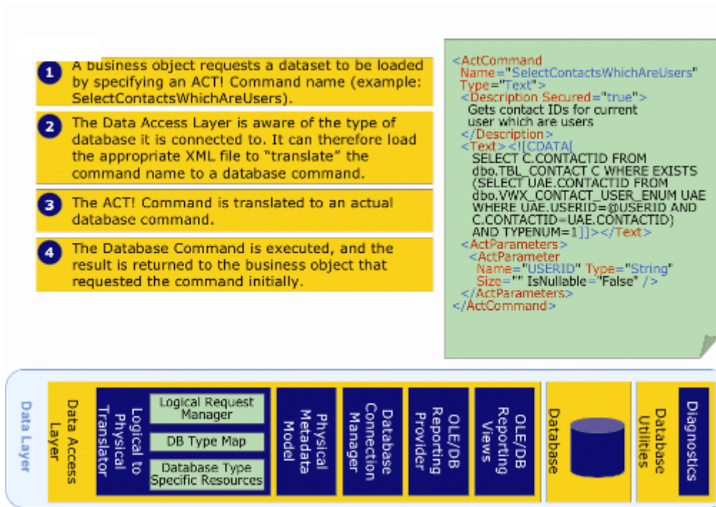
Figure 2: Example Showing the Use of the Data Access Layer
