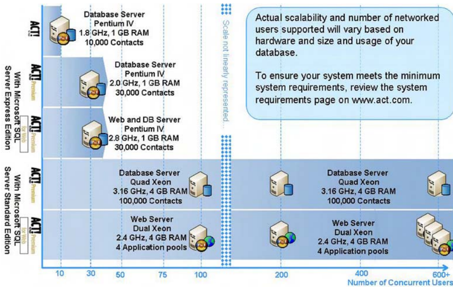
Figure 22: Sage ACT! Scalability
