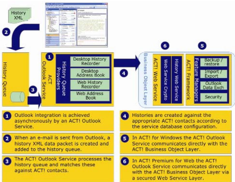
Figure 14: Outlook Email Integration
