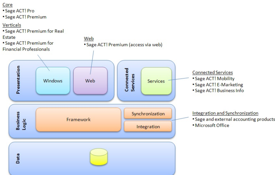
Figure 1: Sage ACT! Architecture Layered Tiers
