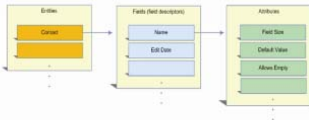
Figure 6: Entities, Fields, and Attributes
