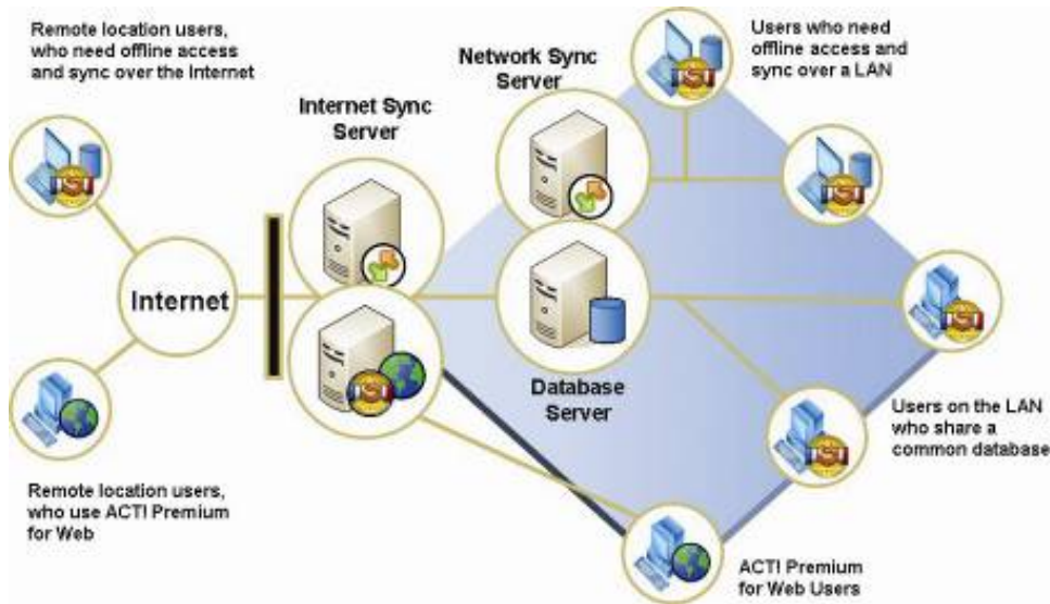
Figure 20: Sage ACT! Premium / Sage ACT! Premium (access via web) Mixed Deployment
