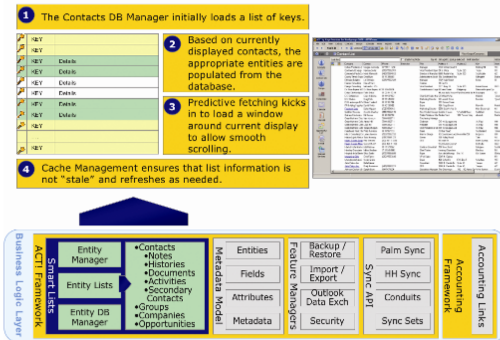
Figure 3: Example Showing the Use of the Business Logic Layer – Smart Lists
