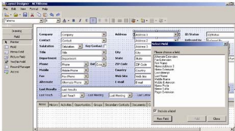
Figure 8: Layout Design
