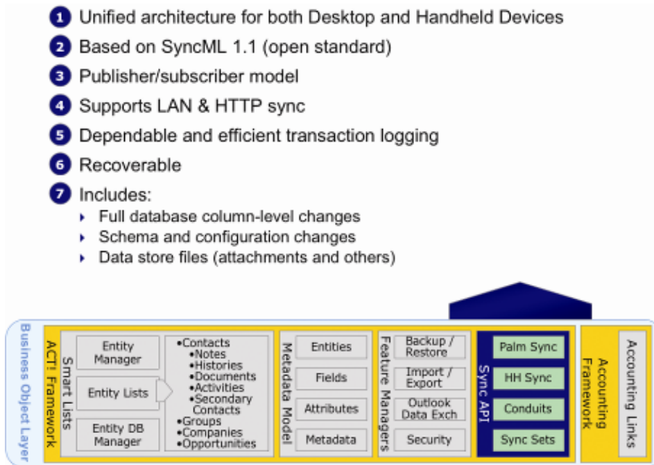
Figure 23: Sage ACT! Synchronization
